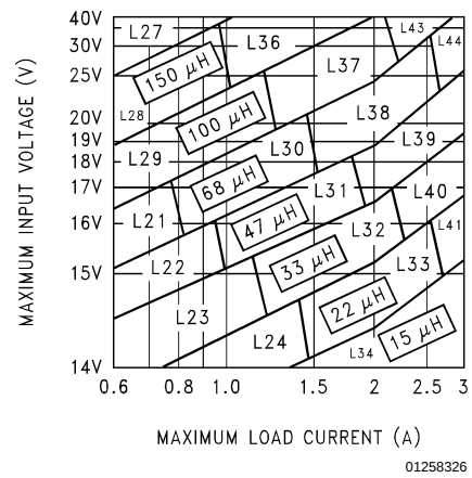
FIGURE 6. LM2596-12
