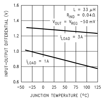
Dropout Voltage
