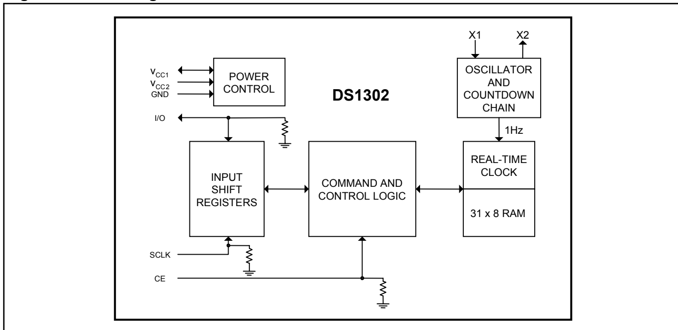
Figure 1. Block Diagram
