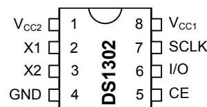
DIP (300 mils)
