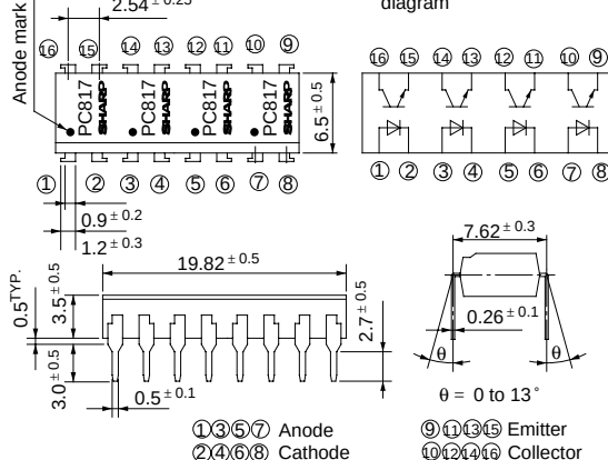
Internal connection diagram
